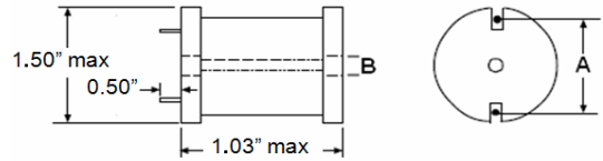
B: Clearance Hole For 8/32 Screw With Washer
