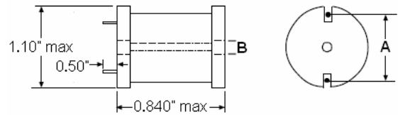
B: Clearance Hole For 4/40 Screw With Washer
