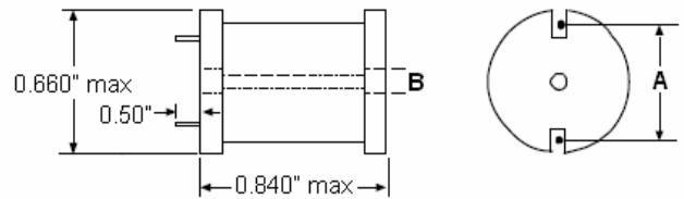
B: Clearance Hole For 4/40 Screw With Washer
