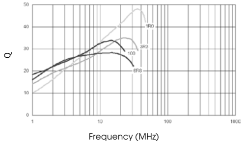
Q vs. Frequency Characteristics
